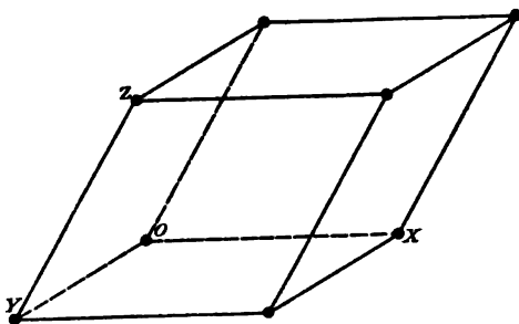
FIG. 27. The unit cell derived from \Gamma_0 . The edges of this unit are of unequal lengths and make unequal angles with one another.
